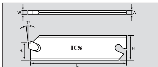
ADJUSTABLE BLADES
