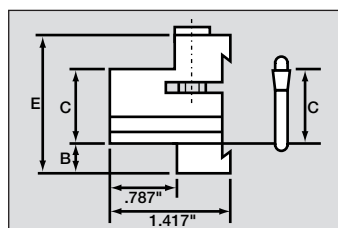
TOOL BLOCKS
